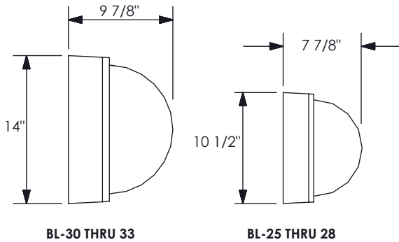
TYPICAL FIXTURE DIMENSIONS
