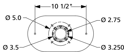
BL-44 THRU 49 MOUNTING DETAIL
